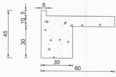
SECTION OF WELL PLATFORM
