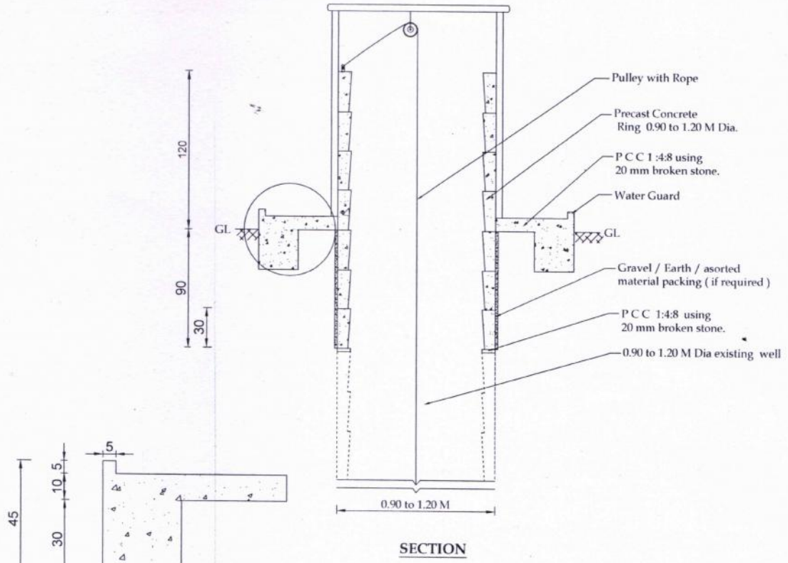
SECTION OF WELL PLATFORM
