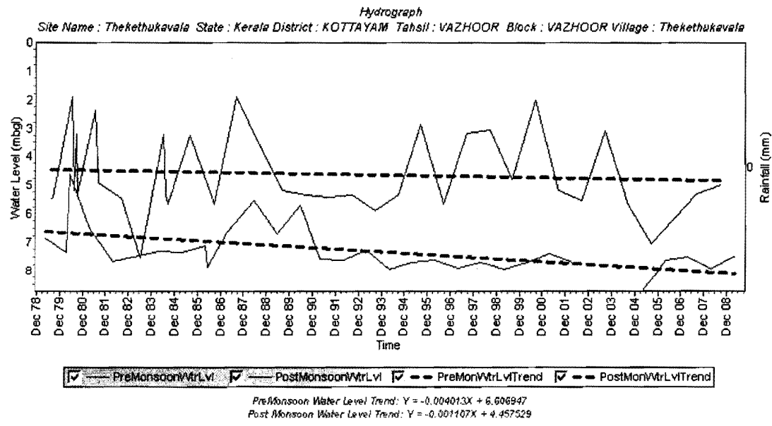
Figure 3-8 Hydrograph of GMMW Tapping Phreatic Aquifer in Laterites at Thekethukavala, Kottayam District
