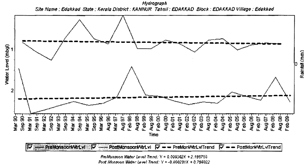
Figure 3-7 Hydrograph of GMMW Tapping Phreatic Aquifer in Laterites at Edakkad, Kannur District
